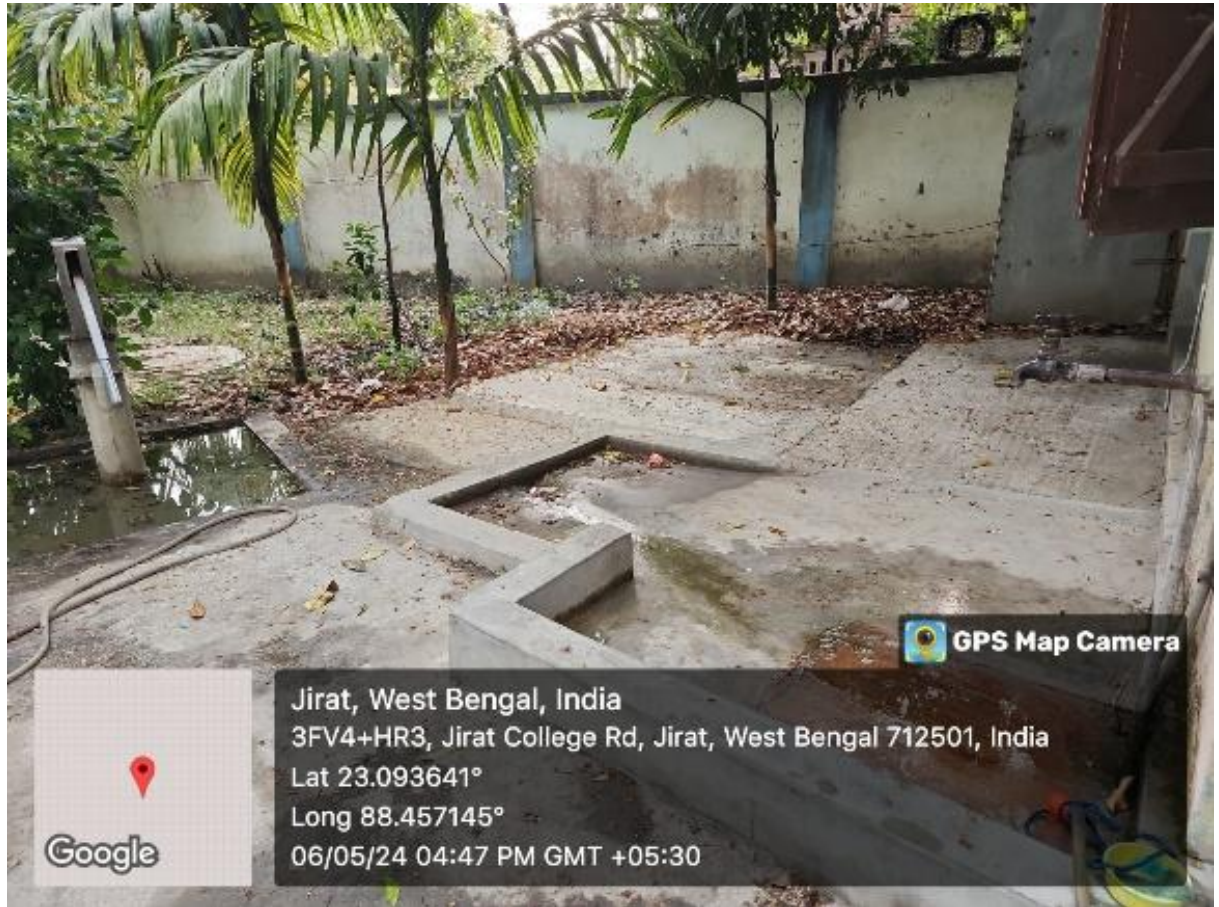
Vertical Filter Chamber With Silt Chamber (1)
